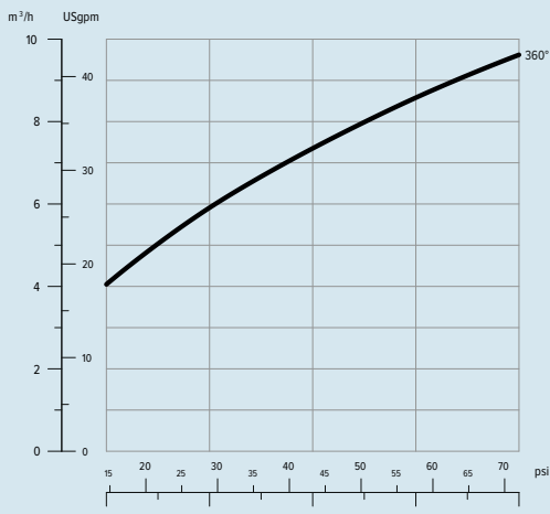
Pressure/Flow
