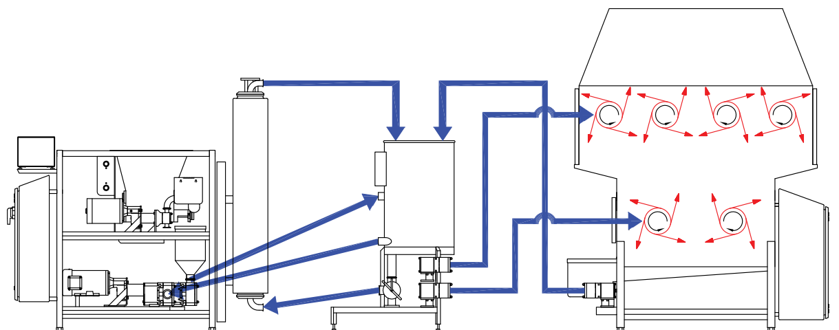
WILEVCO SERIES 9 MIXER AND 4.5x6 CRYOLATOR
