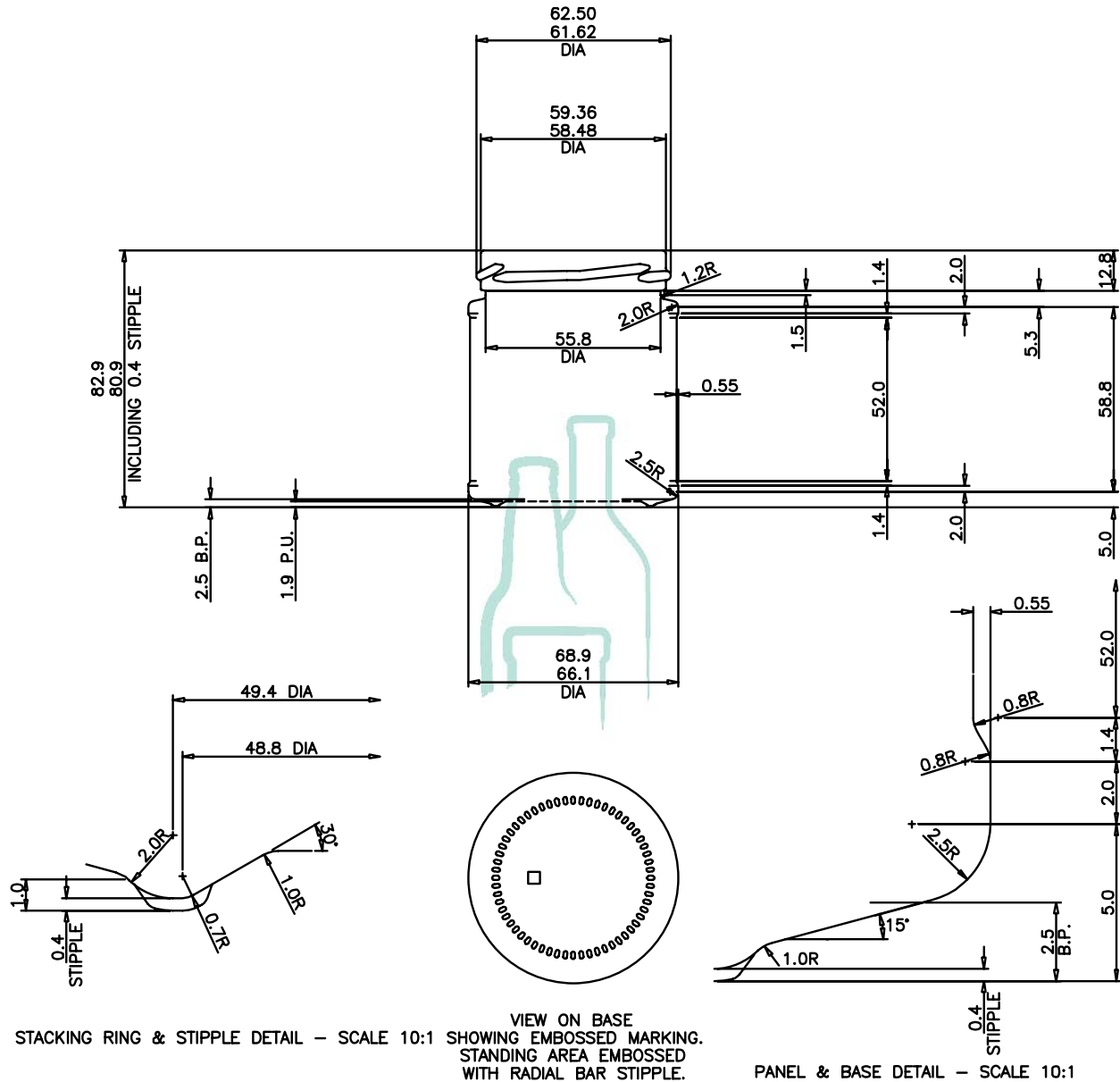
PANEL & BASE DETAIL - SCALE 10:1
