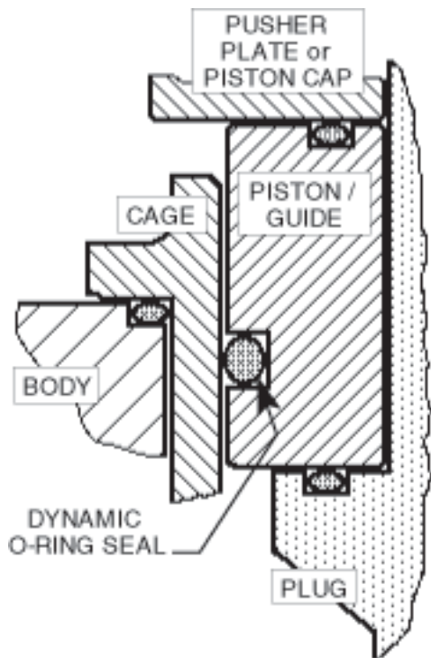
O-RING DYNAMIC SEAL
