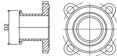
Clamp
