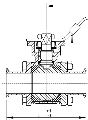
Clamp ball valve with high platform 高平台快装球阀
